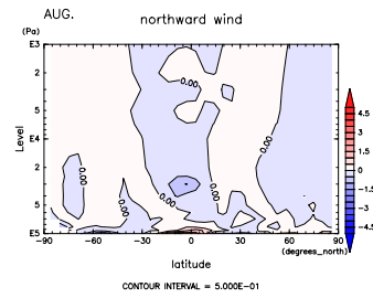
Figure 634: V at Aug. by DCPAM
