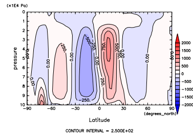
Figure 334: MSF at Apr. by DCPAM
