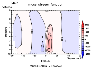
Figure 331: MSF at Mar. by DCPAM
