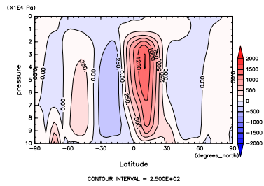
Figure 331: MSF at Mar. by DCPAM
