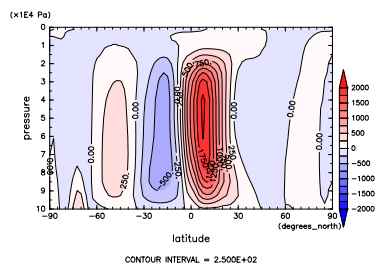
Figure 332: MSF at Mar. by NCEP
