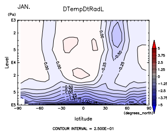
Figure 841: (\partial T/\partial t)_{LW} at Jan. by DCPAM
