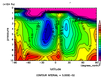
Figure 449: RH at Jun. by NCEP
