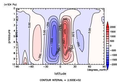
Figure 335: MSF at Apr. by NCEP
