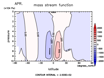
Figure 334: MSF at Apr. by DCPAM
